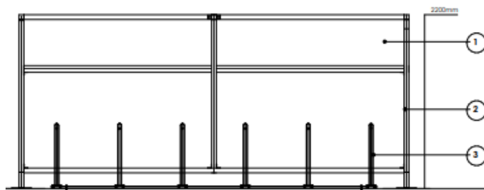
FRONT ELEVATION 1:20
