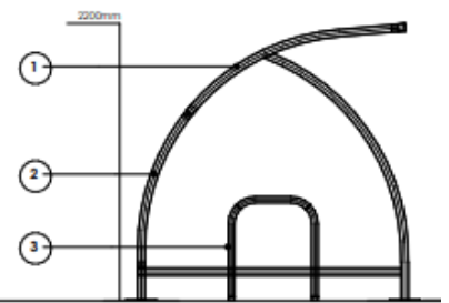
SIDE ELEVATION 1:20
