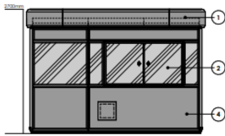
SIDE 1 ELEVATION 1:25
