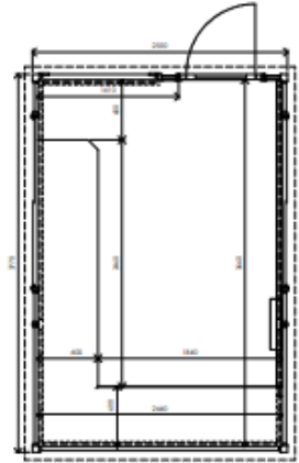
FLOOR PLAN 1:25
